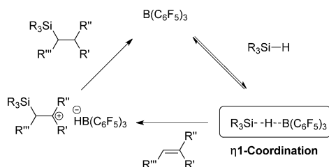
Scheme 2. B(C_6F_5)_3 -catalyzed alkene hydrosilylation.
