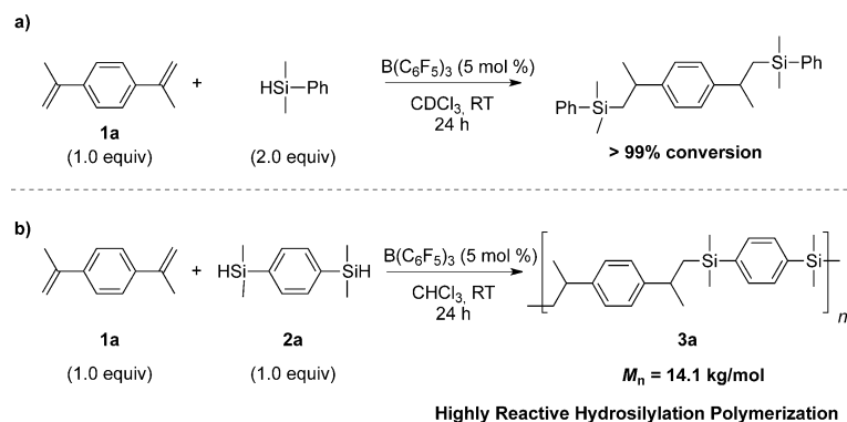
Scheme 3. a) Highly reactive B(C_6F_5)_3 -catalyzed hydrosilylation and b) hydrosilylation polymerization.
